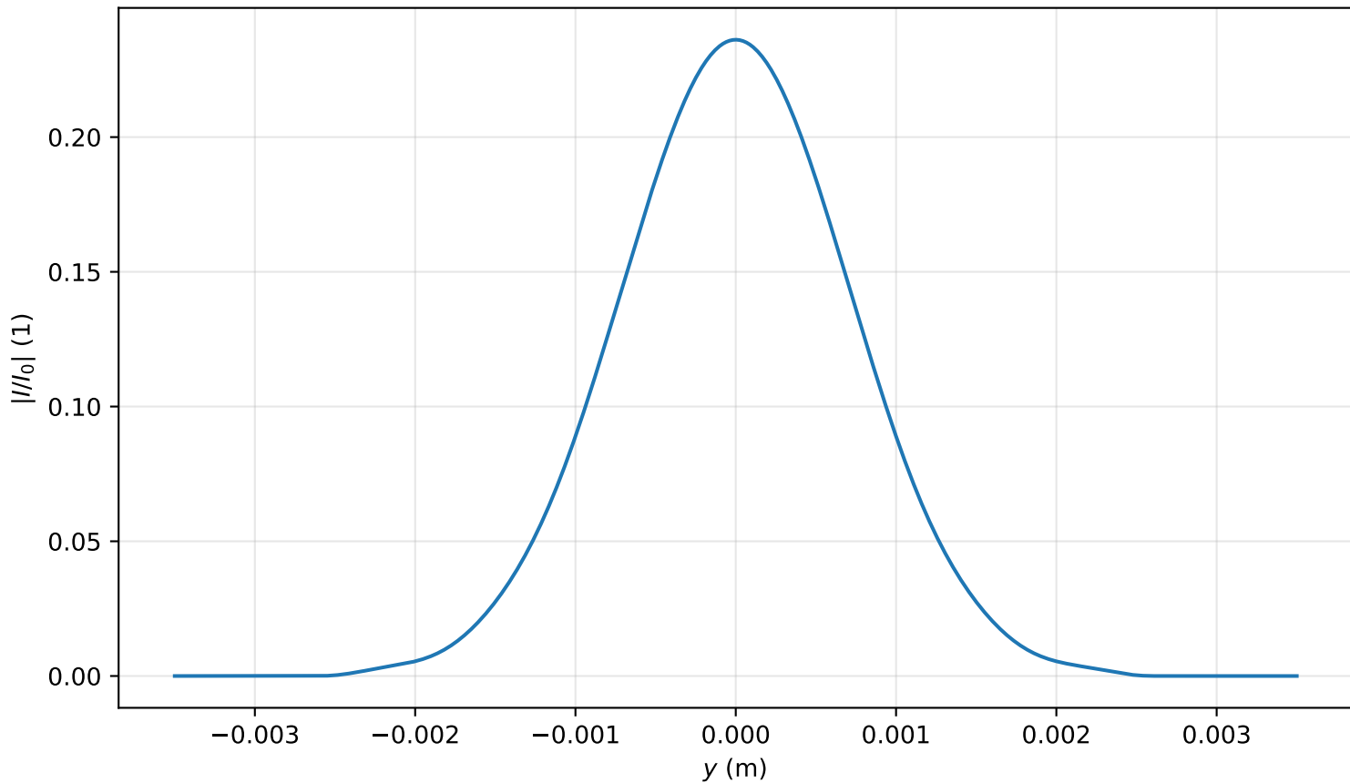
Intensity profile I(x=0, y, z=3.821)/I_0 , P_{in}=0.1P_{cr} , artificial time
